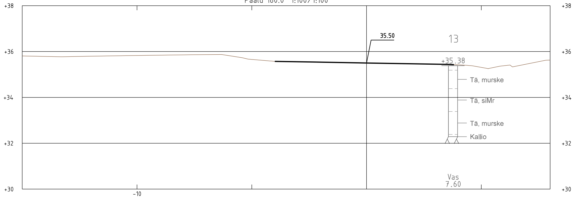
Paalu 180.0 1:100/1:100
