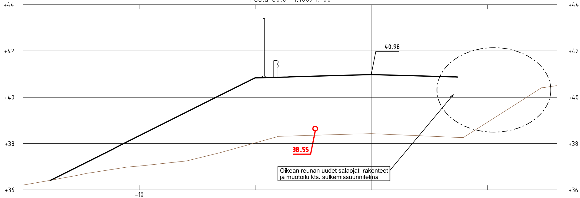
Paalu 80.0 1:100/1:100
