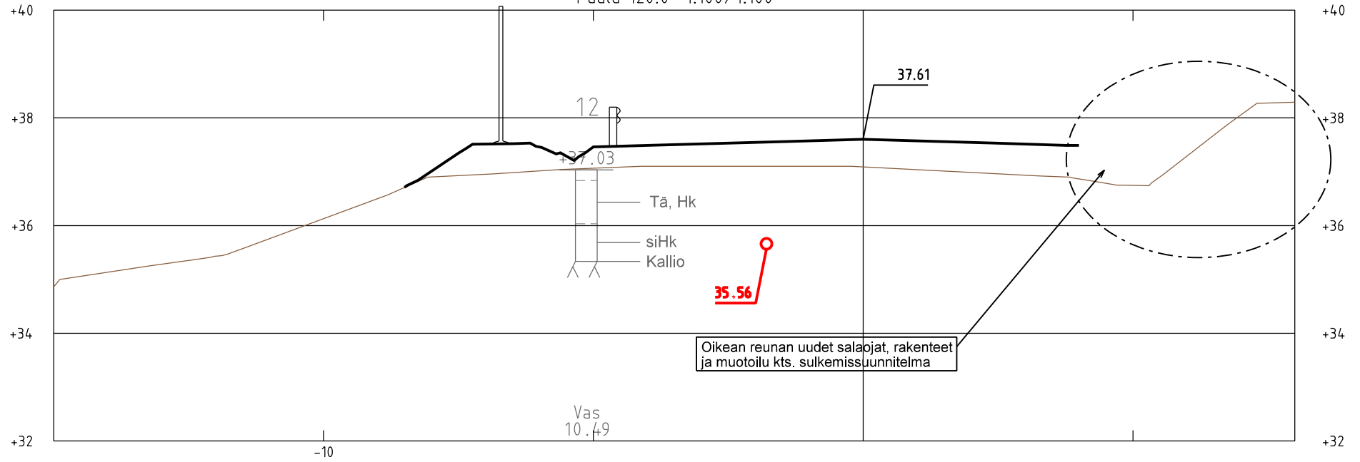
Paalu 120.0 1:100/1:100
