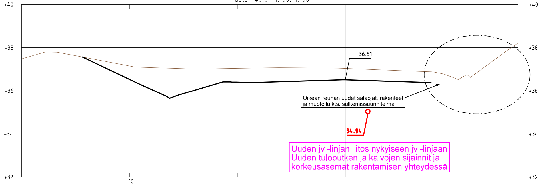
Paalu 140.0 1:100/1:100
