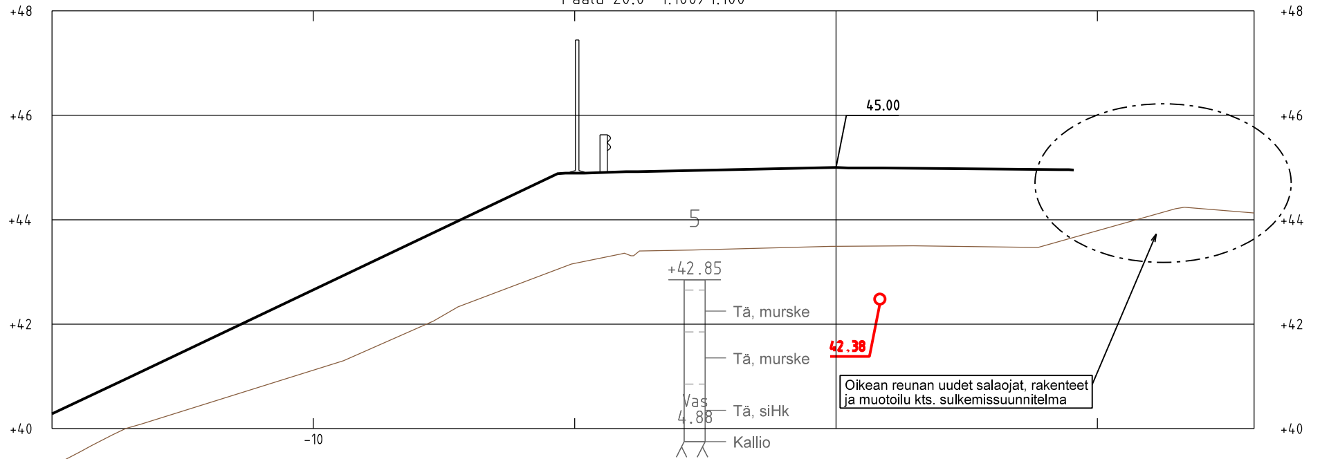
Paalu 20.0 1:100/1:100
